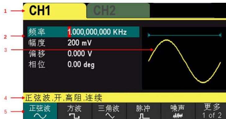
Figure 4.3 User interface
